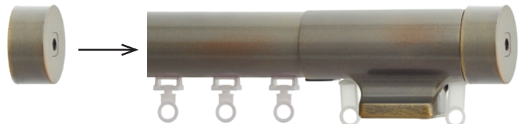
new 1 3/8" Transitional Cuff / Finial Adapter PO138CUFF QS138CUFF 3/4" L x 1 1/2" W • Metal, Available in any of our 35 Portfolio Hand Painted Finishes, 5 Quick Ship Wood & Resin Finishes or PTH Perfect Match™ • Required to adapt your 1 3/8" Today's Traditional or Heritage Classics Finials to work with Metal Traverse, sold separately
